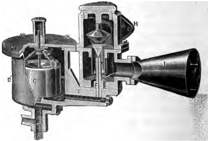
FIG. 153.—The "Phenix" Daimler Carburettor. A is the gasoline needle valve; B, the weighted controlling levers; C, the float; D, the float chamber; E, the gasoline supply tube; F, the spraying nozzle; G, the "mushroom" spray deflector; H, the port leading to the cylinder chamber; I, the air inlet. The air entering the mixing chamber follows the course of the arrows.
